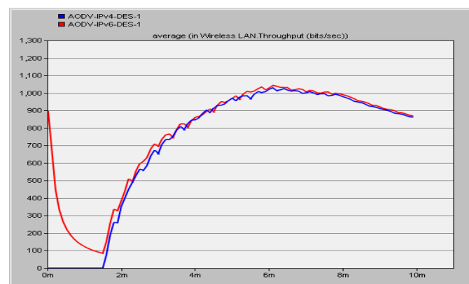
Fig.3 illustrate the average WLAN throughput (bit/sec)
