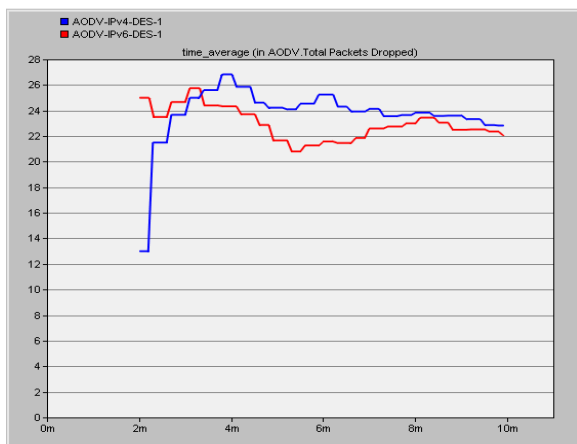
Fig.5 illustrate the total packets dropped (pkts)
